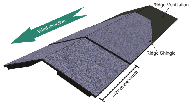
Fig 1.53 - Over-lapped Ridge Shingle.
