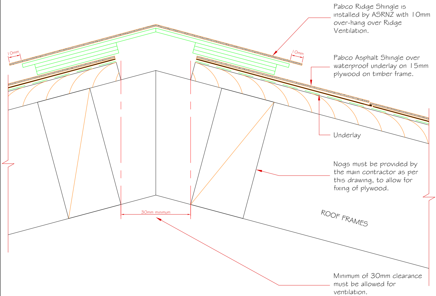
AIR-FLOW DIAGRAM @ 1:5
