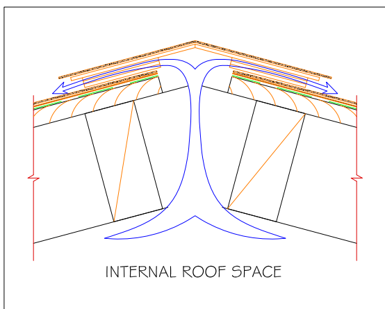
AIR-FLOW DIAGRAM @ 1:5
